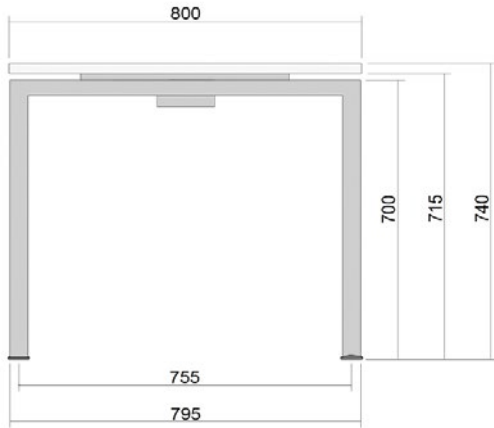
800 Desk Leg
