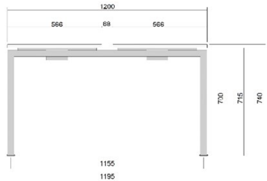
1200 Bench Leg
