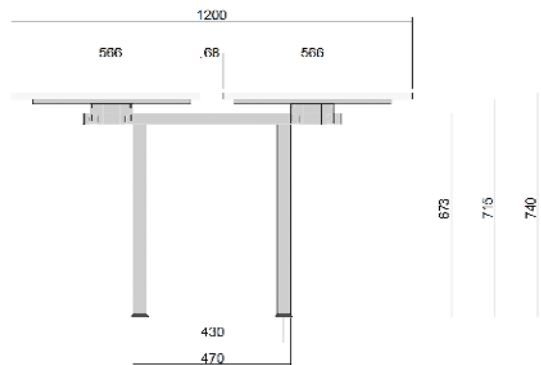
1200 Intermediate Bench Leg
