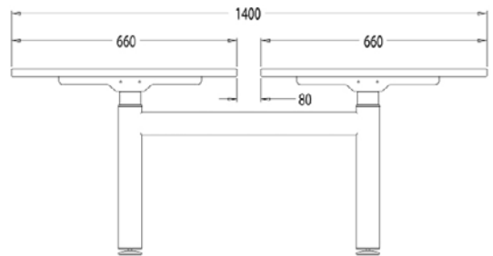
Screen Gap 80mm - Ref: 'P'
