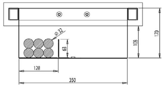
High-Capacity Cable Tray
