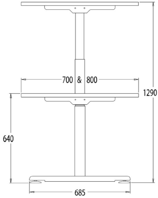
Desk with Rounded Feet and Glides
