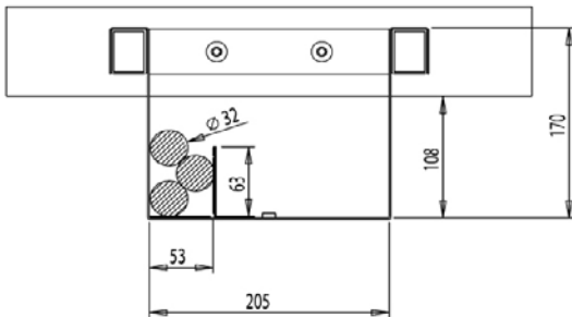
Standard Cable Tray
