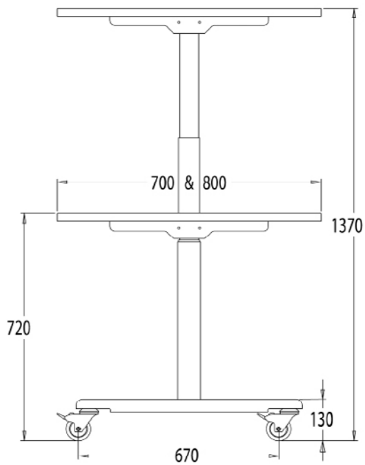
Desk with Rounded Feet and Castors
